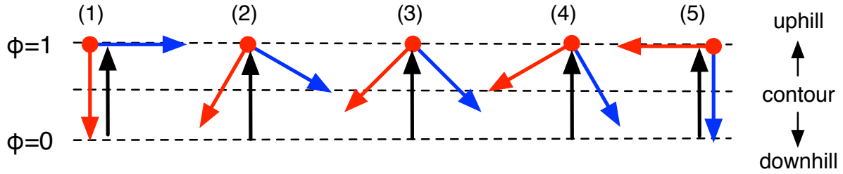
Figure 1: Gradient of the scalar function \phi in 2D case
