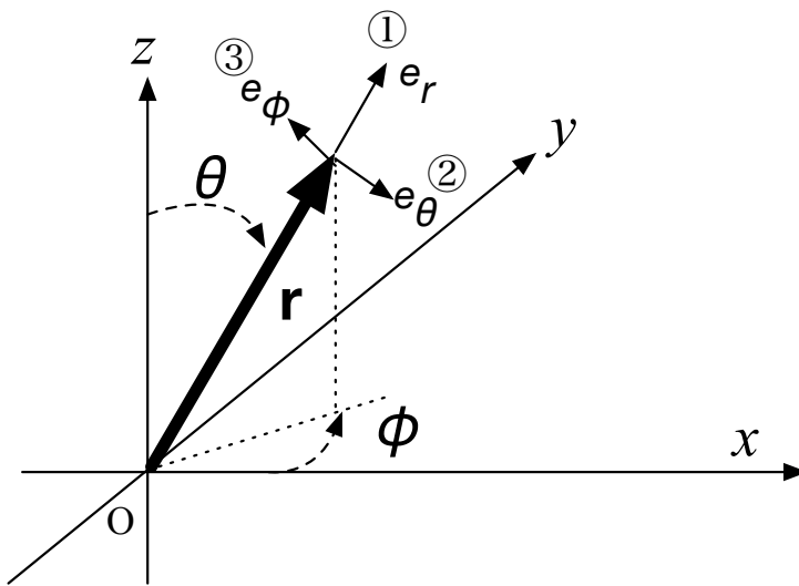
Figure 3: spherical coordinate
